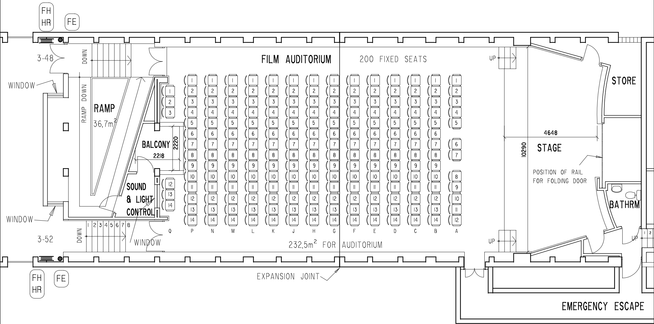
FLOOR PLAN OF DR MIRIAM MAKEBA AUDITORIUM
